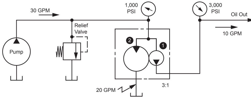
Figure 3. Using a Rotary Pressure Intensifier with Unequal Sections.
