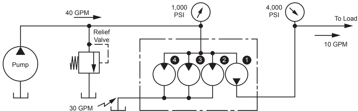
Figure 4. Pressure Intensification with a 4-Section Flow Divider.
