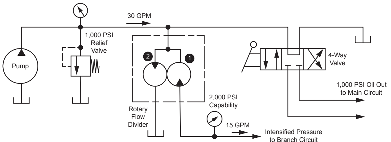
Figure 2. Intensified Pressure in One Branch of a Hydraulic Circuit.
